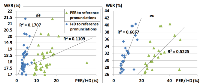
Fig. 5. Correlation betw. PER/I+D to qualified dictionary and WER.
