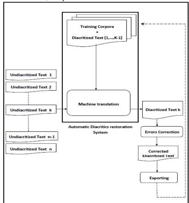
Figure 1. Iterative Diacritization Process
