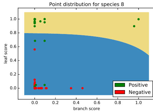
Fig. 4. Distributions of negative and positive samples formed based on the branch and leaf scores for species id 8
